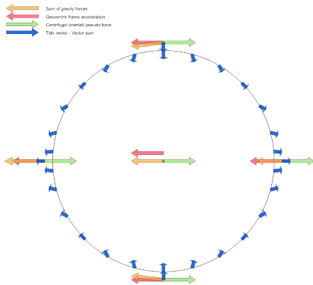
Fig. 4 - Tidal force explained. Orange arrows show gravitational field, red acceleration of the reference frame, green fictitious centrifugal acceleration (opposite to reference frame acceleration), blue is sum of gravitational and centrifugal acceleration.
