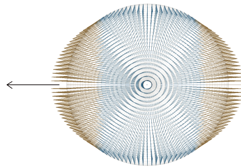
Fig. 5 Tidal force on Earth due to Moon only, view from above north pole, moon little above equator. Arrow points toward moon. Brown vectors are pointing outside, blue vectors are pointing inside.
