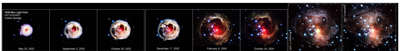
Fig. 3 - V838 Mon outburst light echo, illuminating interstellar dust, that could have been thought of as a dark matter...
